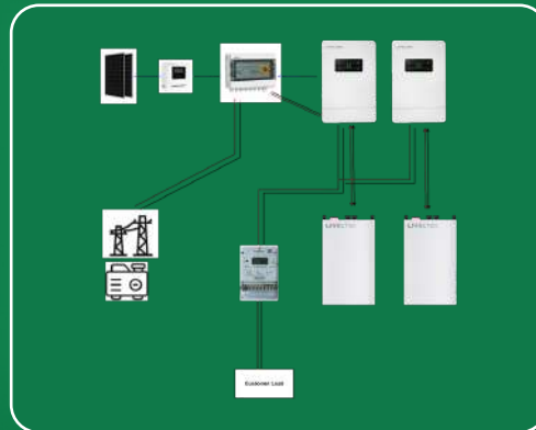
5.12kwh battery ②
